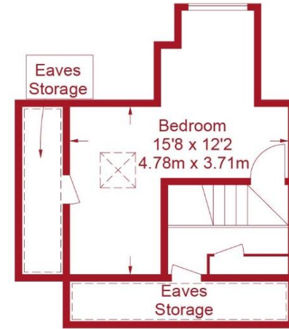
Second Floor 334 sq ft / 31.0 sq m (Including Eaves Storage / Reduced Headroom)
